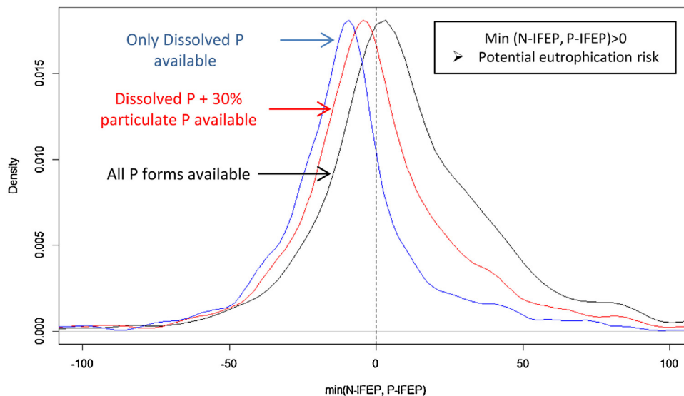
Fig. 6. Density functions of eutrophication risk \min(\text{N-IFEP}, \text{P-IFEP}) in 2210 headwater catchments under 3 hypotheses.
