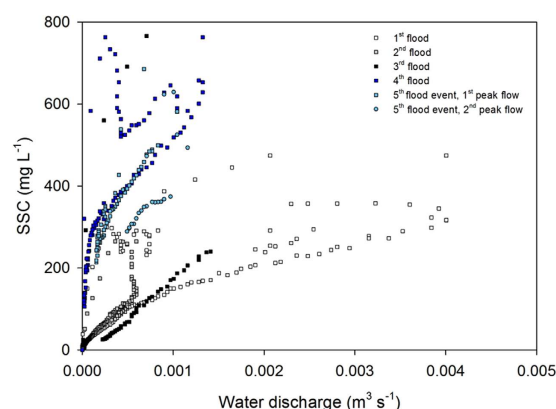
Figure 4. Water discharge and suspended sediment concentrations (SSC) for the five monitored flood event at the tile drain outlet of the Brépinière (BR) station. This original graph was created using SigmaPlot 12.5 software ( http://www.sigmaplot.co.uk/products/sigmaplot/produpdates/prod-updates18.php ).
