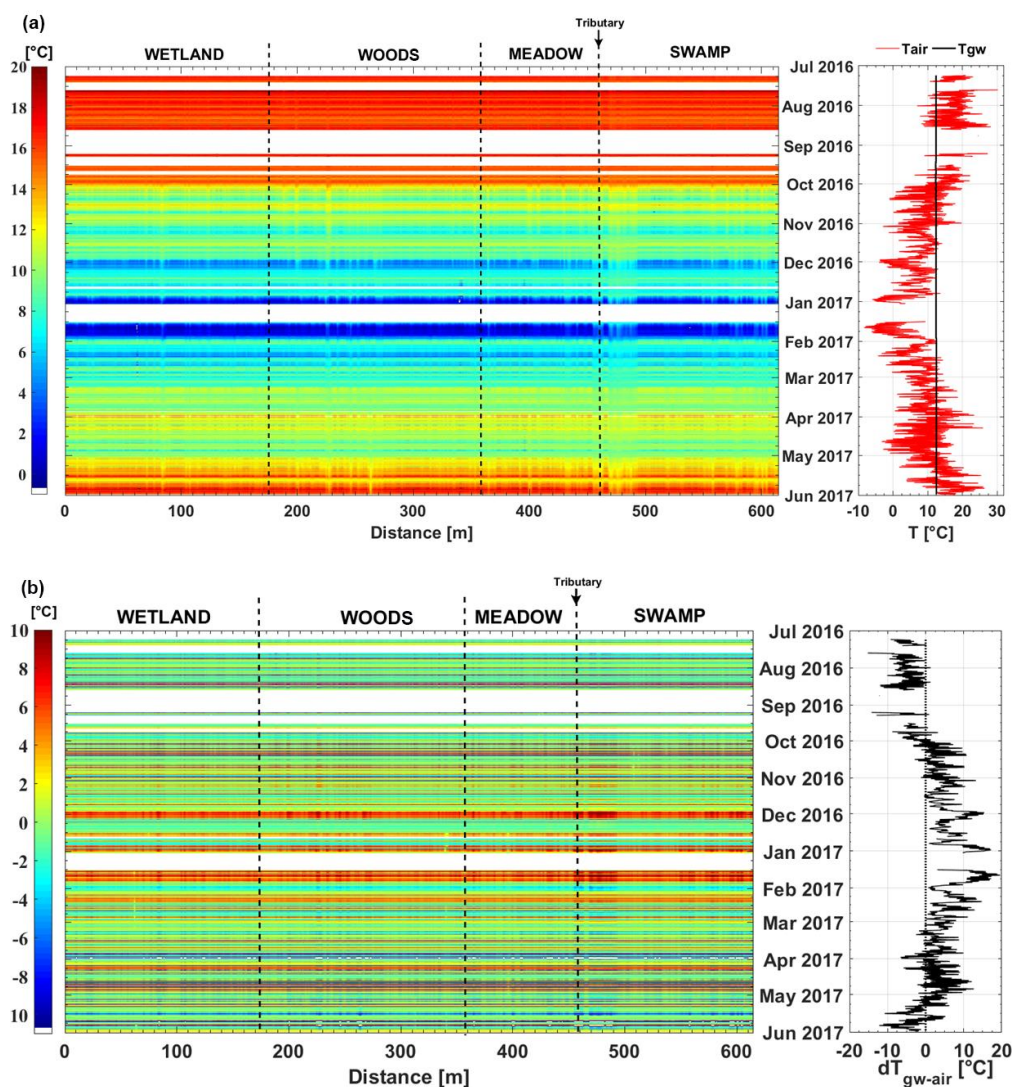
Figure 5. Spatiotemporal evolution of (a) streambed temperature ( T_{\text{sed}} ) in the Petit Hermitage compared to dynamics of air and groundwater temperature ( T_{\text{air}} and T_{\text{gw}} , respectively) and (b) the difference between sediment and air temperature ( dT_{\text{sed-air}} ) compared to dynamics of T_{\text{gw}} minus T_{\text{air}} ( T_{\text{gw-air}} ). White bands indicate missing data.
